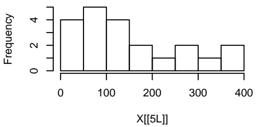
Histogram of X[[5L]]
