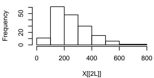
Histogram of X[[2L]]
