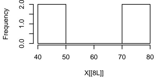
Histogram of X[[8L]]
