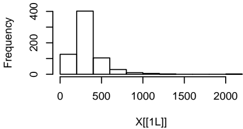
Histogram of X[[1L]]
