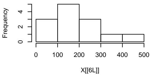
Histogram of X[[6L]]
