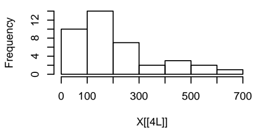
Histogram of X[[4L]]
