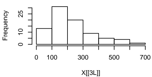
Histogram of X[[3L]]
