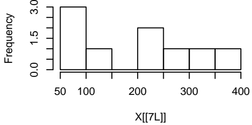
Histogram of X[[7L]]
