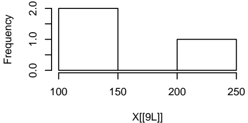
Histogram of X[[9L]]
