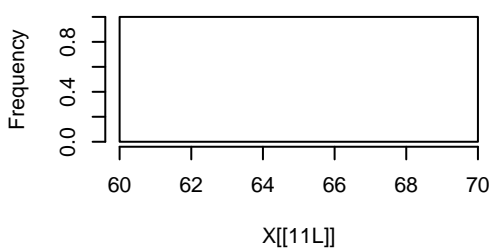
Histogram of X[[11L]]
